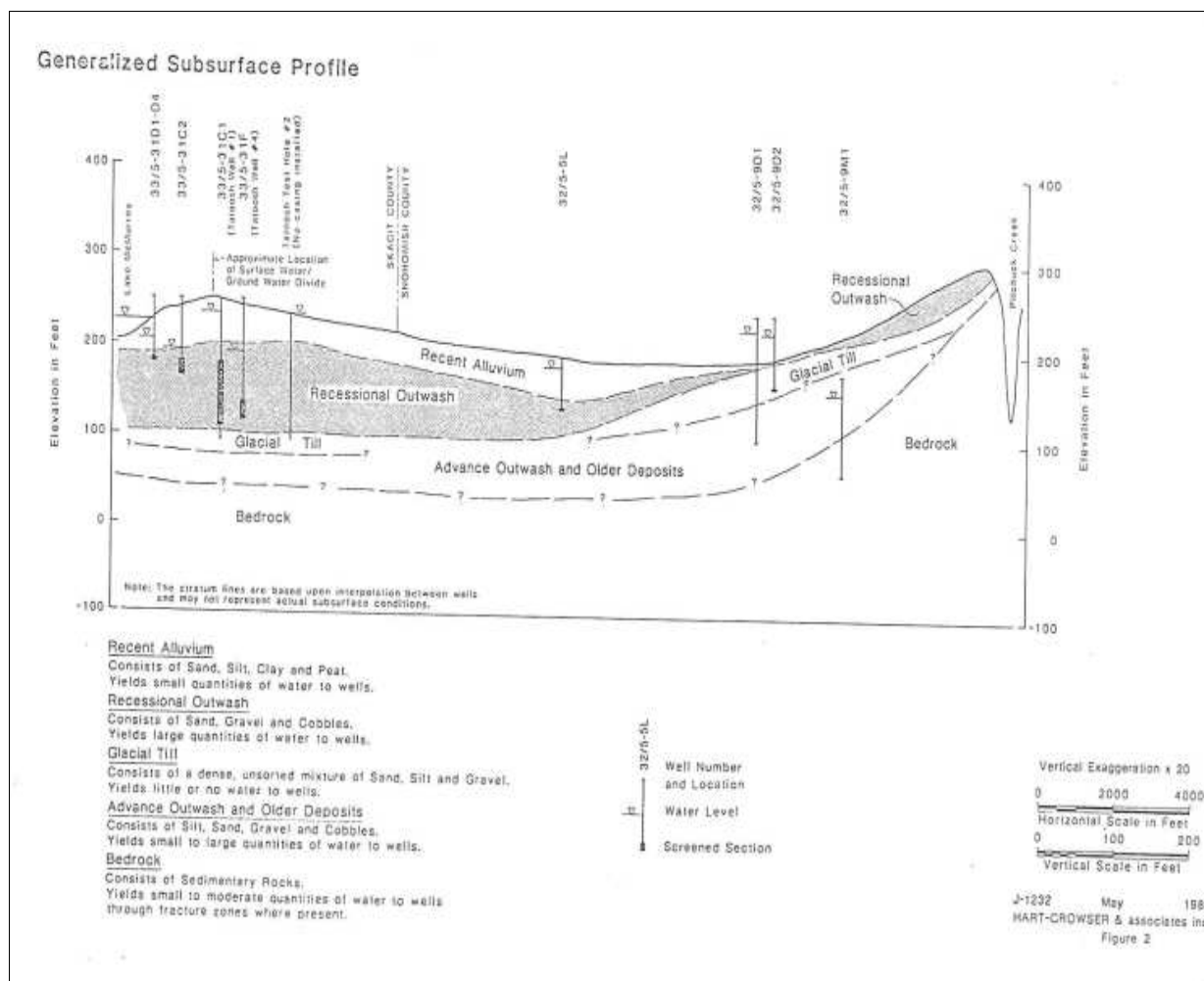
Figure 8 – Subsurface Profile Showing Groundwater Divide
