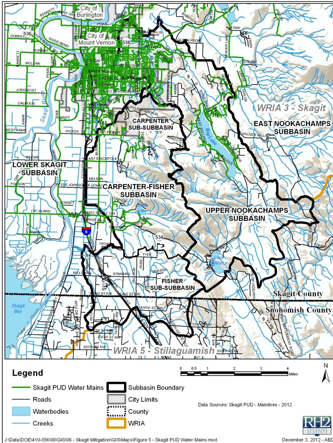
Figure 5 – Existing Skagit PUD Water Mains
